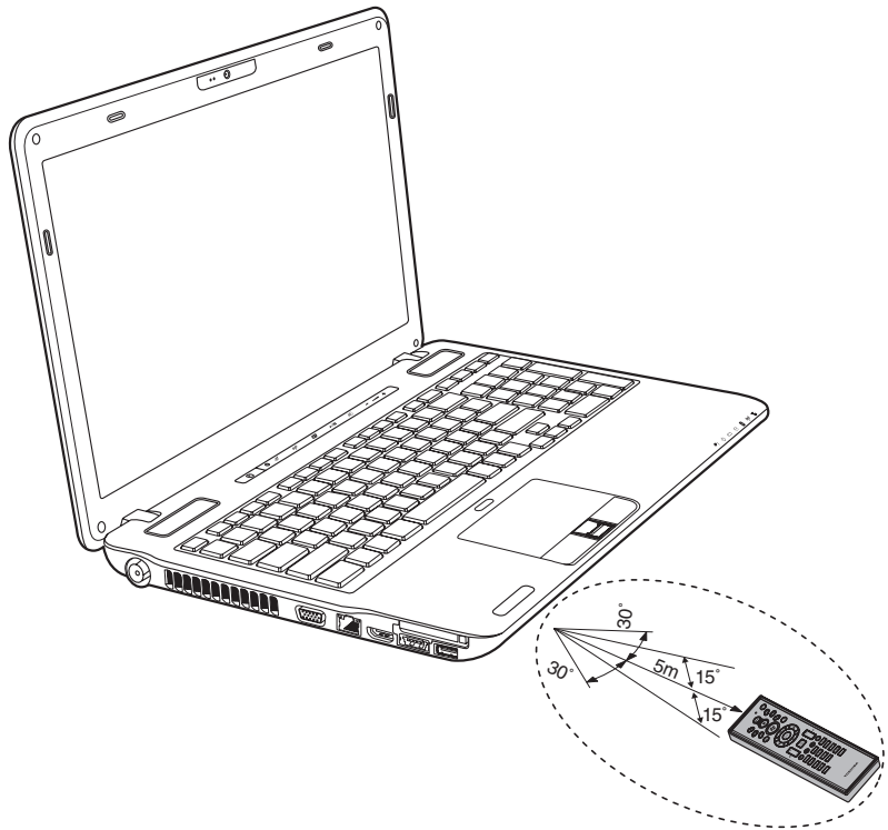
Figure 2-12 Operational range of the remote control
