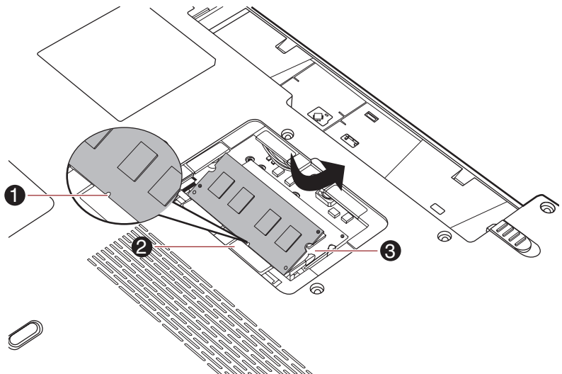
Figure 3-7 Seating the memory module
