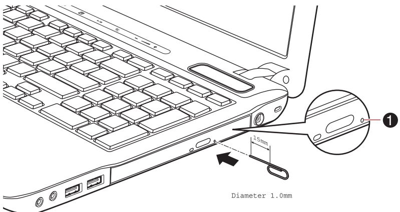
Figure 4-9 Manual release with the eject hole
