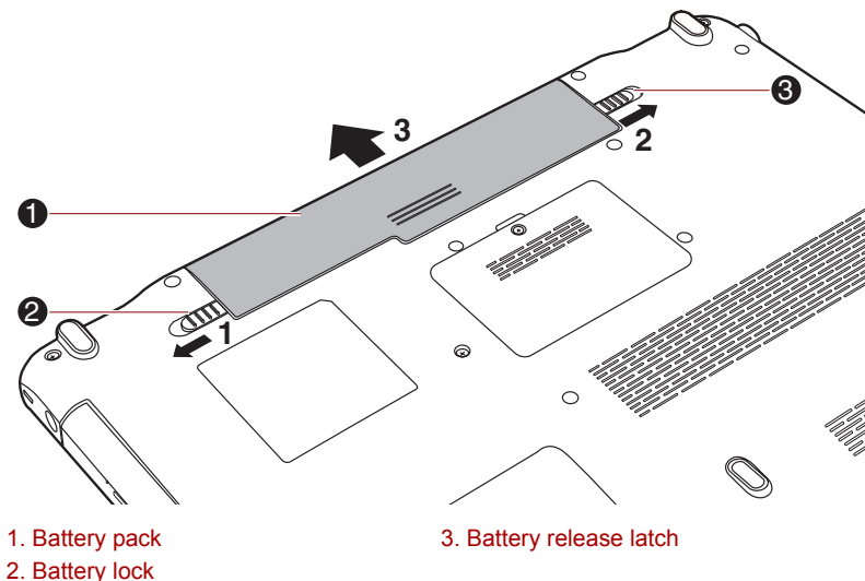
Figure 6-1 Releasing the battery pack
